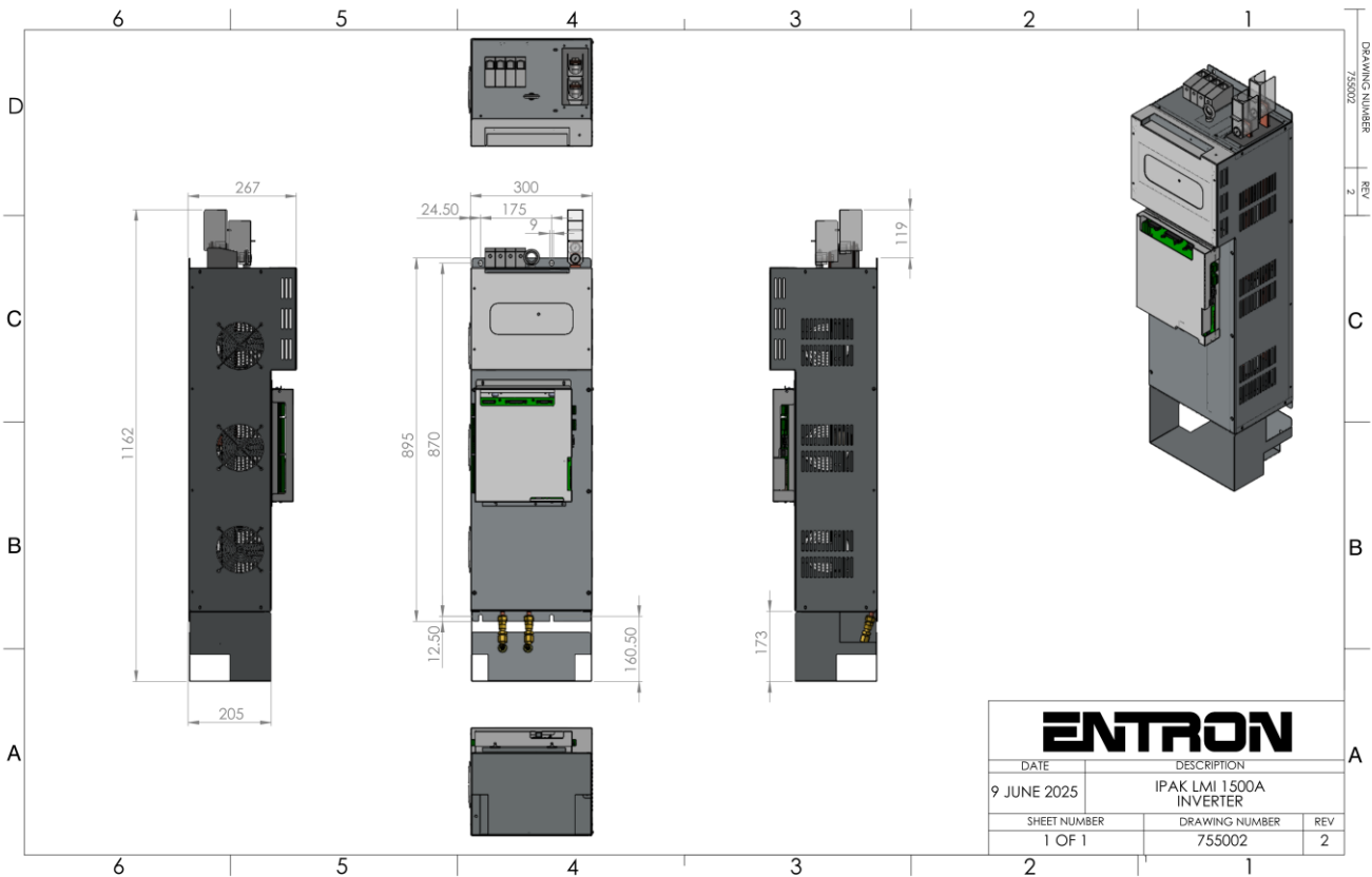
Outline Drawings – Inverter Module:
