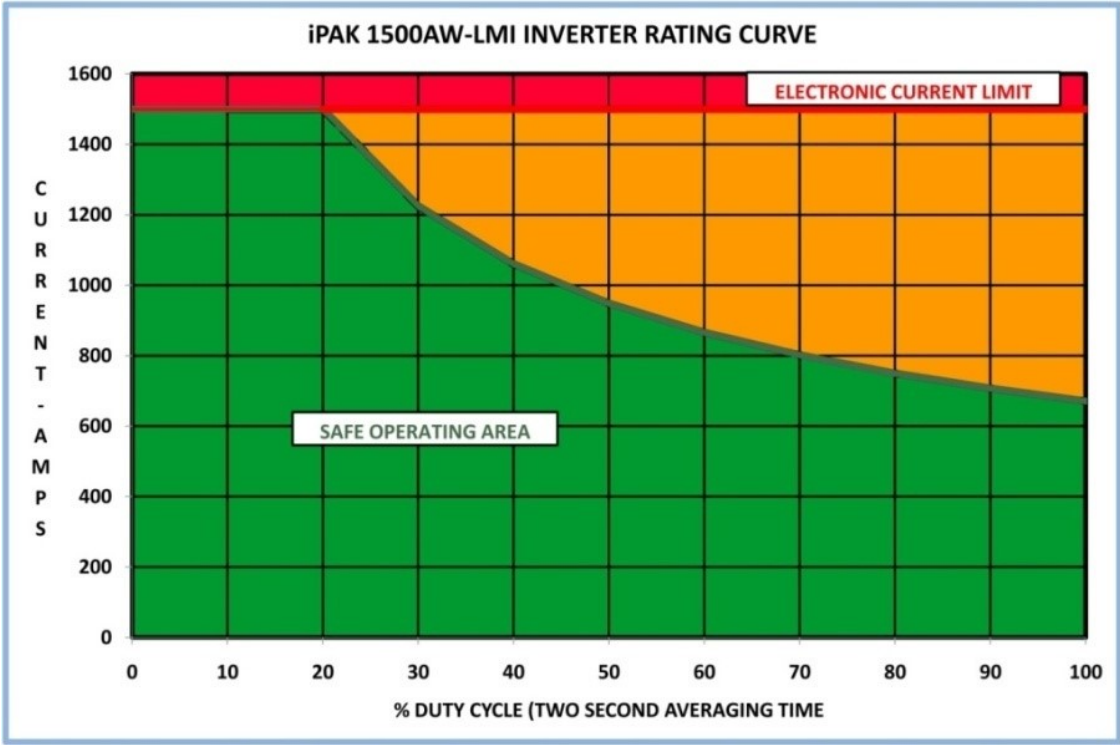
Inverter Rating Curve:
